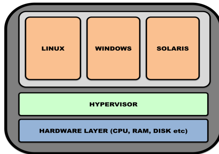
Figure 4 - Platform Virtualization
